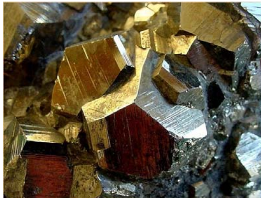
Figure 16: Crystals of pyrite in the form of a cube (left) and pyritohedrons (right). Note the fine grooves on the faces of these crystals.
