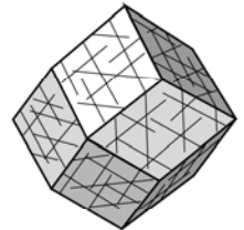
Dodecahedral (6 cleavages -- 12 faces) sphalerite
