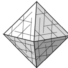
Octahedral (4 cleavages -- 8 faces) fluorite
