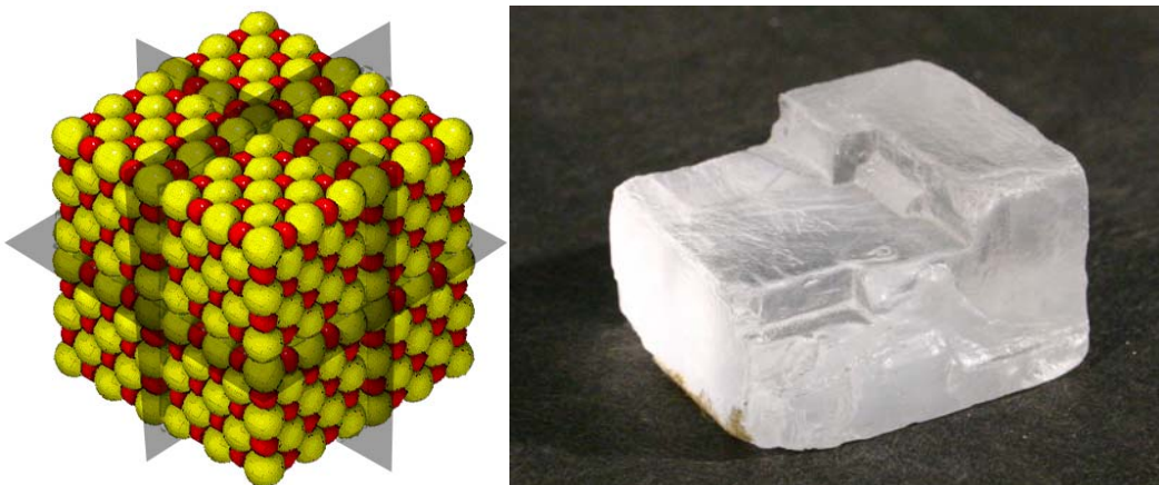
Figure 6: The illustration shows that atoms of sodium (red) and chlorine (yellow) in the mineral halite are parallel to three planes that intersect at 90°. Halite breaks, or cleaves, most easily between the three planes of atoms, so it has three directions of cleavage that intersect at 90°. The photograph illustrates the three directions of cleavage in halite.
