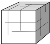
Cubic (3 cleavages at right angles) halite, galena
