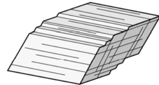
Non-prismatic (2 cleavages not at right angles) hornblende
