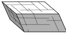
Rhombohedral (3 cleavages, none at right angles) calcite
