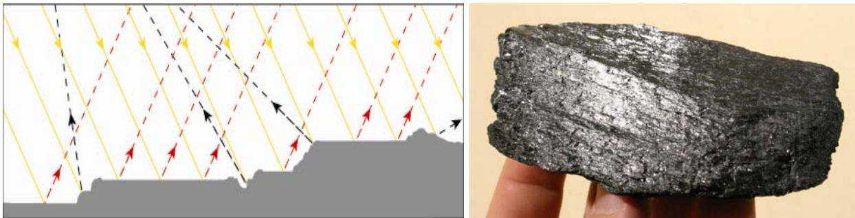
Figure 7: When incoming light rays (yellow lines) strike parallel cleavage surfaces, the rays are all reflected in the same direction (red lines), even though the surfaces are at different elevations. When viewed from that direction, the mineral shines. Rays striking irregular fracture surfaces reflect in many different directions (black lines), causing fracture surfaces to appear duller. The parallel cleavage planes in hornblende shine because the light is reflected in the same direction.
