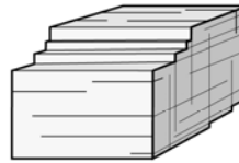
Prismatic (2 cleavages at right angles) feldspars, augite
