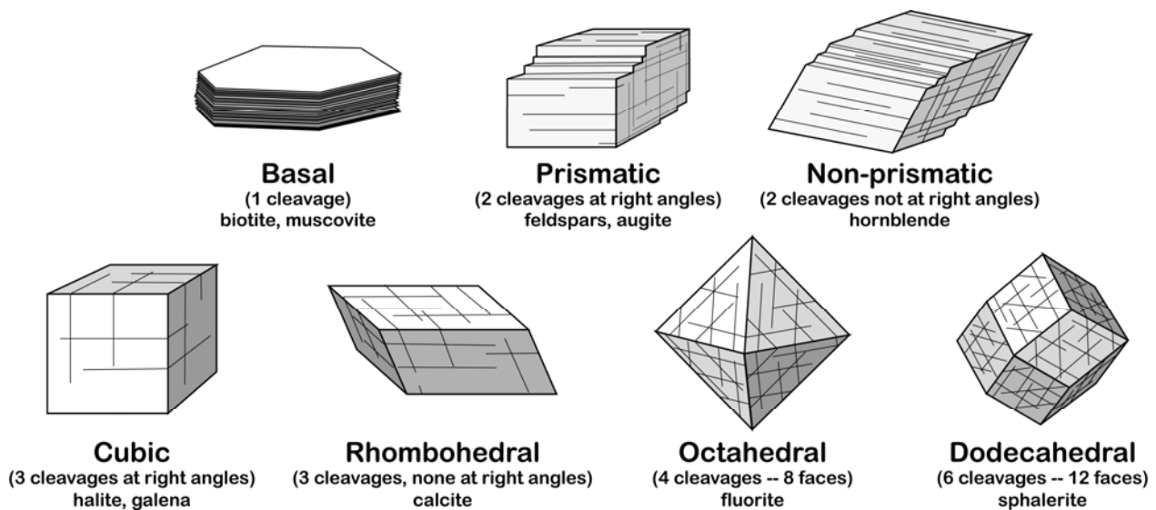
Figure 8: Types of cleavage common in minerals with examples of minerals.
