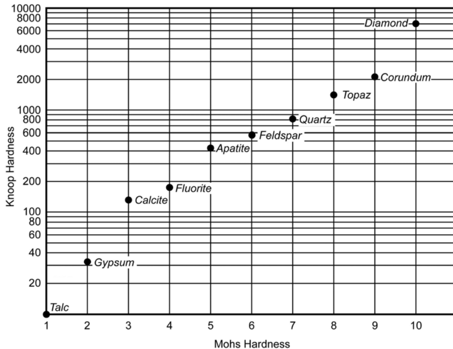
Figure 5: Comparison between Mohs scale hardness and Knoop hardness. Note that the Knoop hardness is shown with a logarithmic scale.
